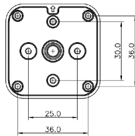
Switch Mounting Details
