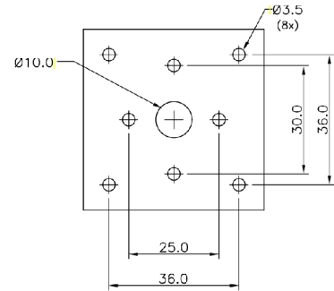
Drilling Plan
